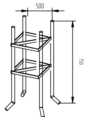
Bolt Cage M24
