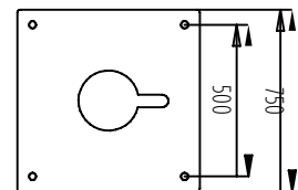
Bolt Cage M24
